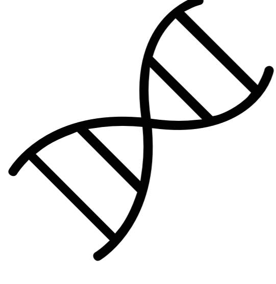
DNA
