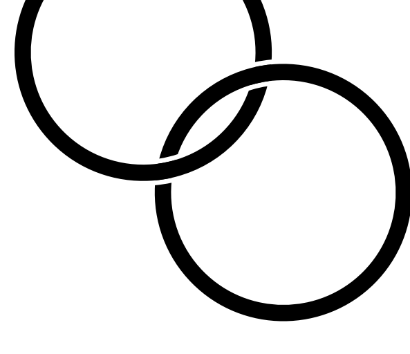
Chains
